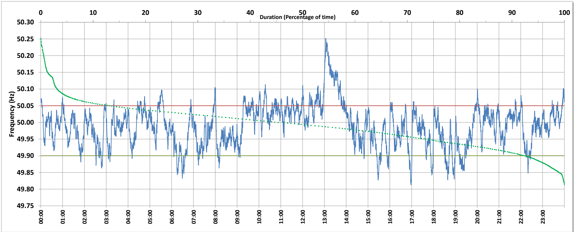
Frequency profile for 02-Aug-2019 (Friday)
