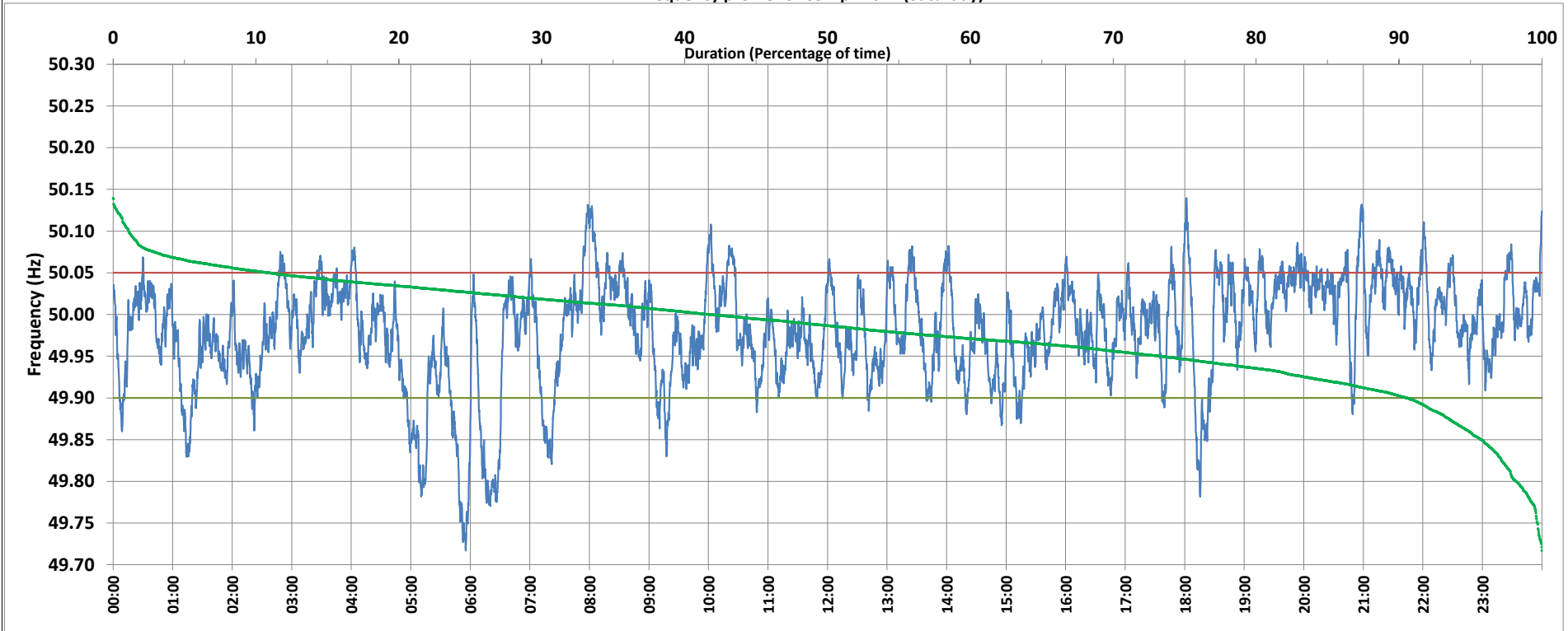
Frequency profile for 03-Apr-2021 (Saturday)
