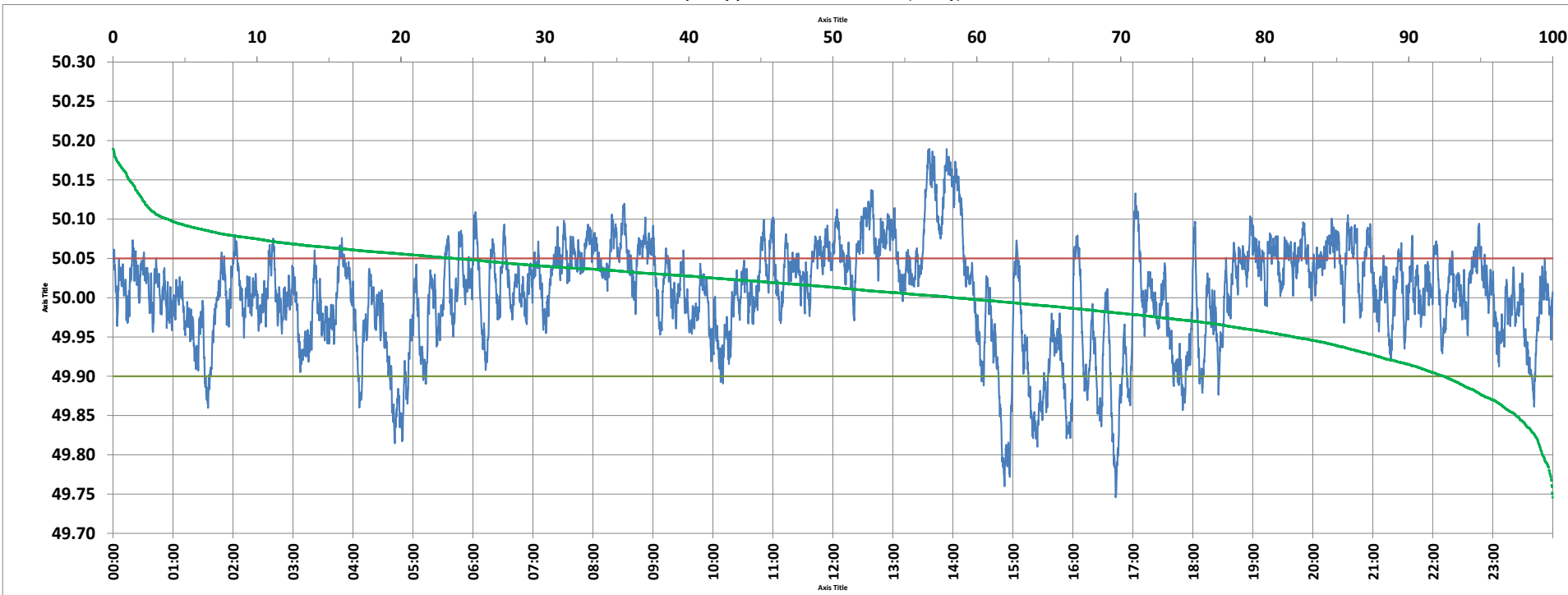
Frequency profile for 05-Nov-2021 (Friday)
