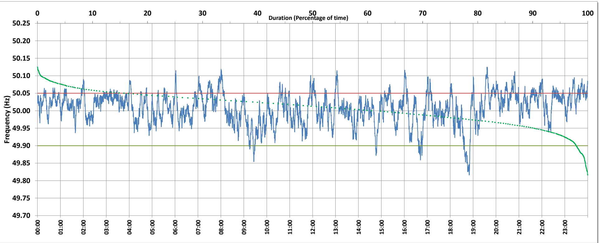
Frequency profile for 07-Sep-2019 (Saturday)
