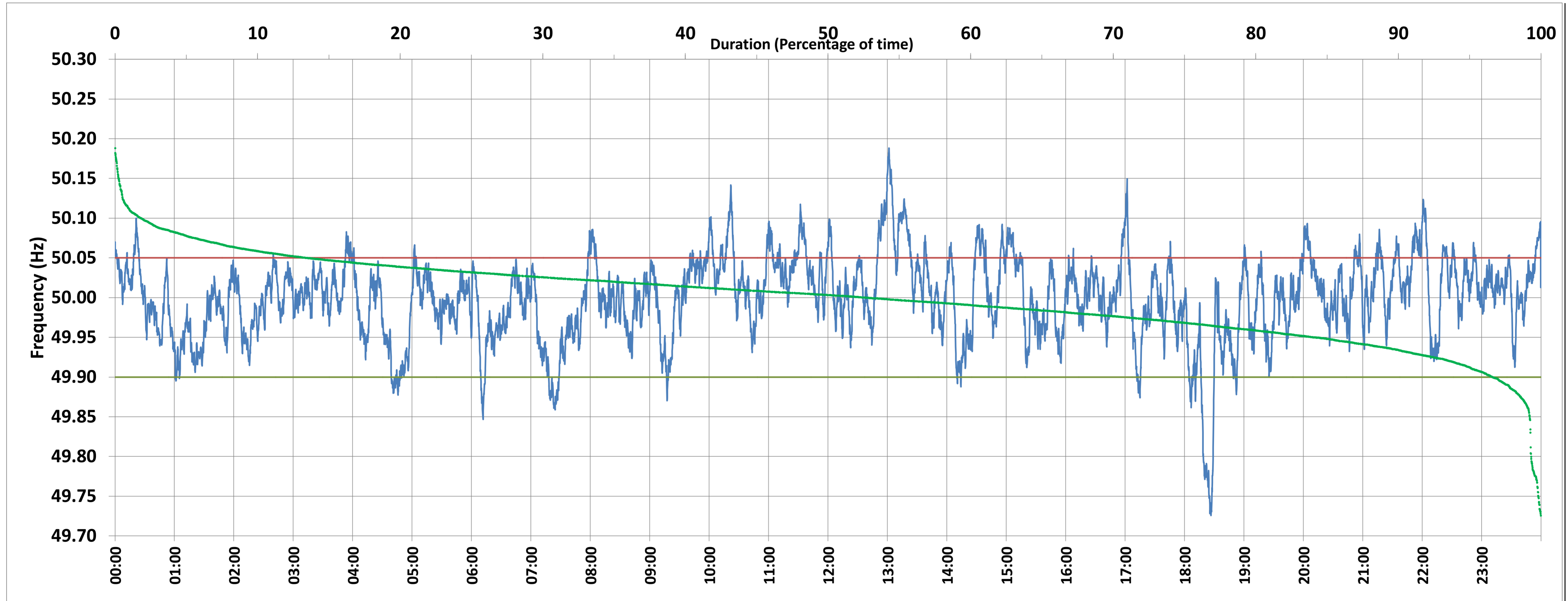
Frequency profile for 11-Aug-2020 (Tuesday)
