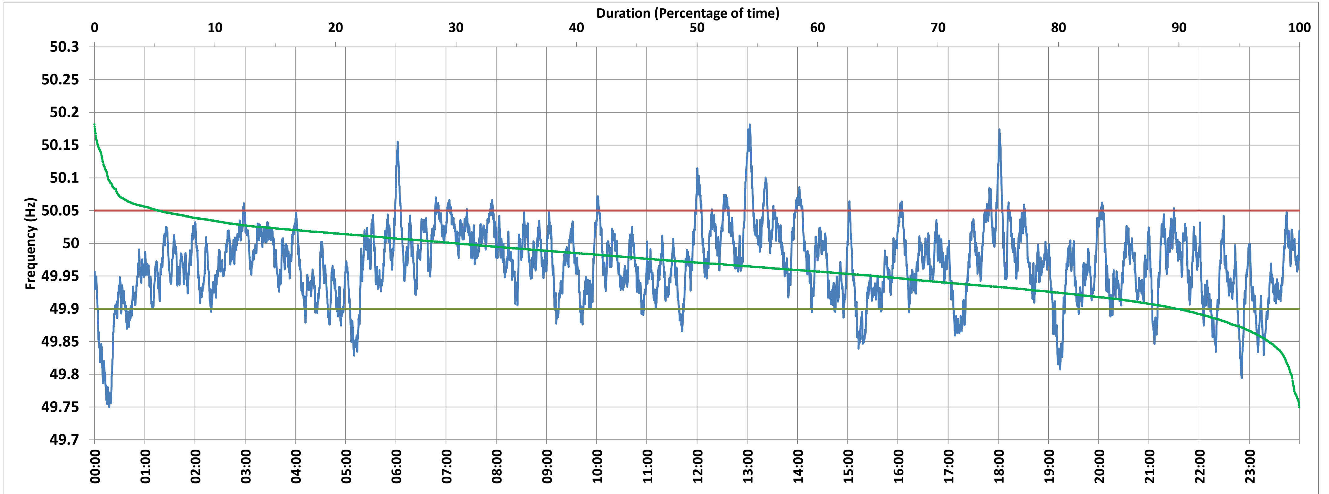
National Grid Frequency Profile for 14-Apr-2018
