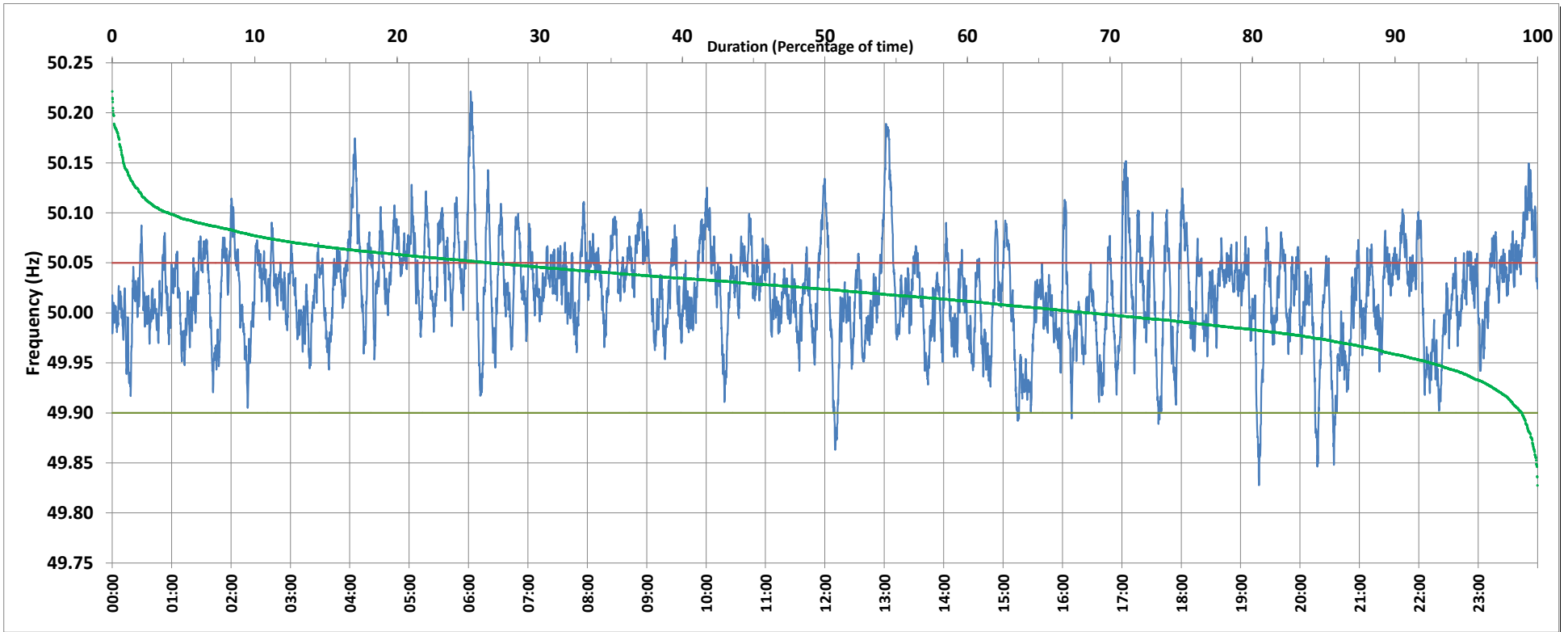
Frequency profile for 23-Nov-2019 (Saturday)
