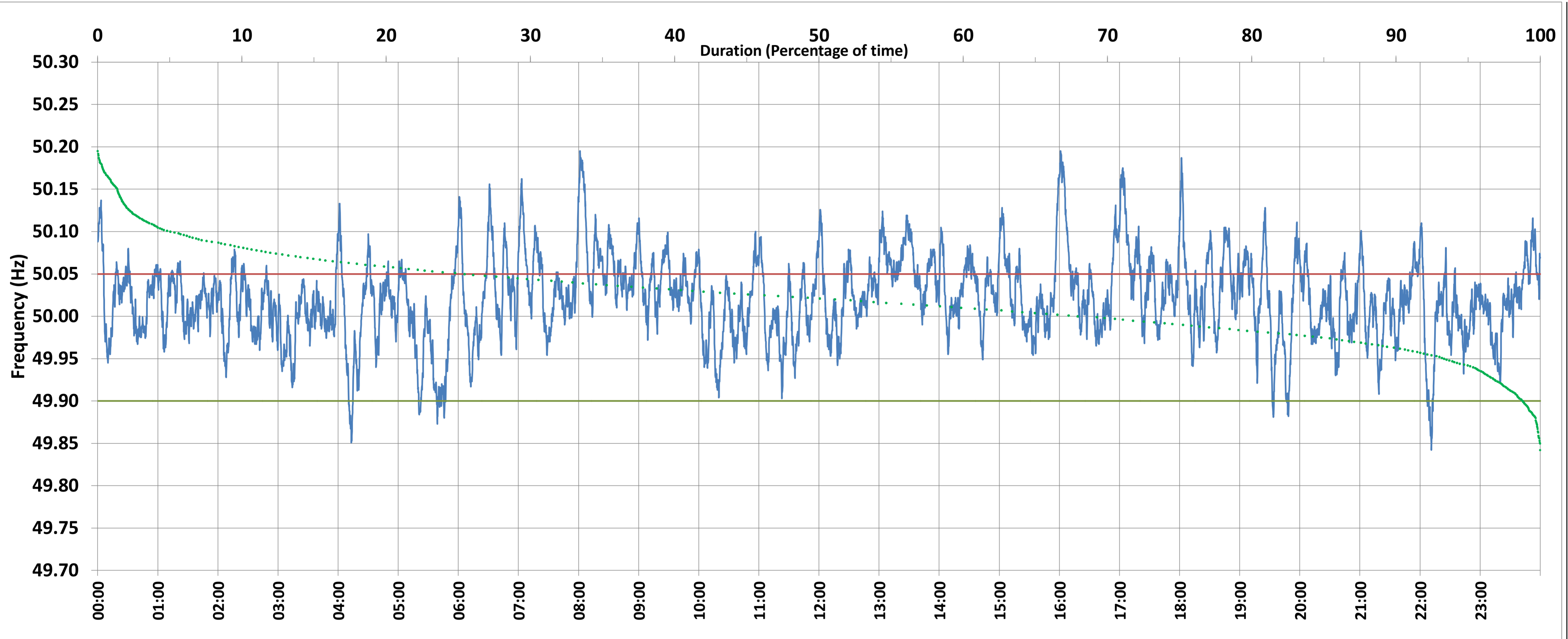
Frequency profile for 24-Jan-2021 (Sunday)
