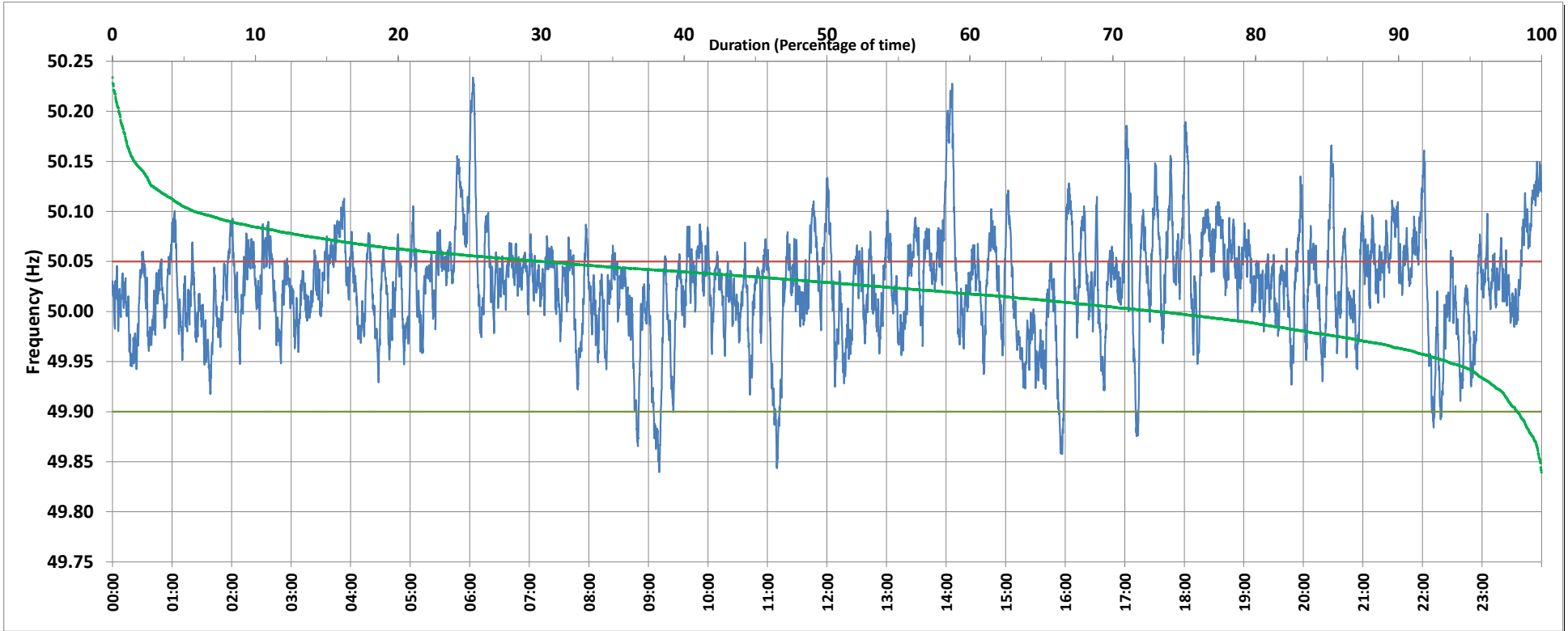
Frequency profile for 24-Nov-2019 (Sunday)
