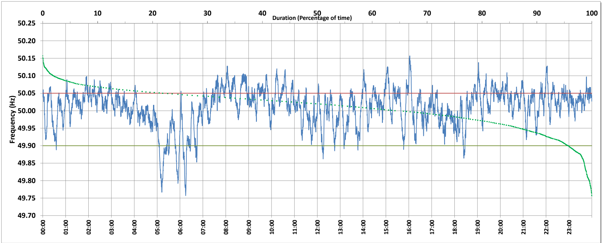
Frequency profile for 25-Aug-2019 (Sunday)
