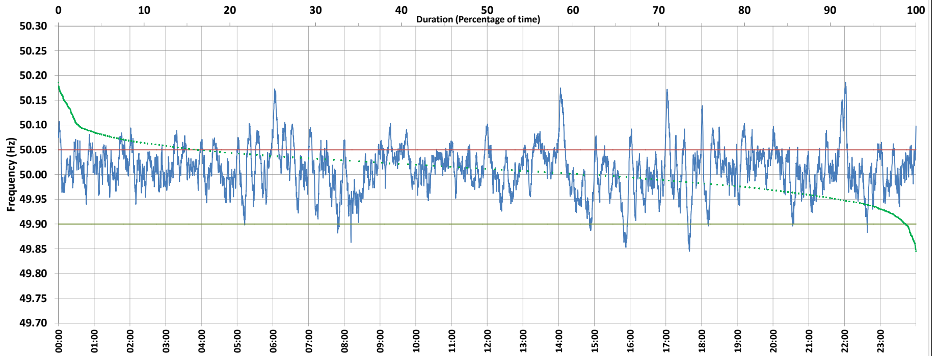
Frequency profile for 27-Dec-2020 (Sunday)
