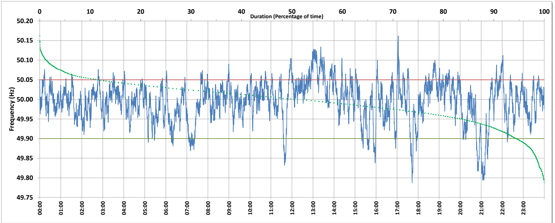
Frequency profile for 31-Oct-2019 (Thursday)
