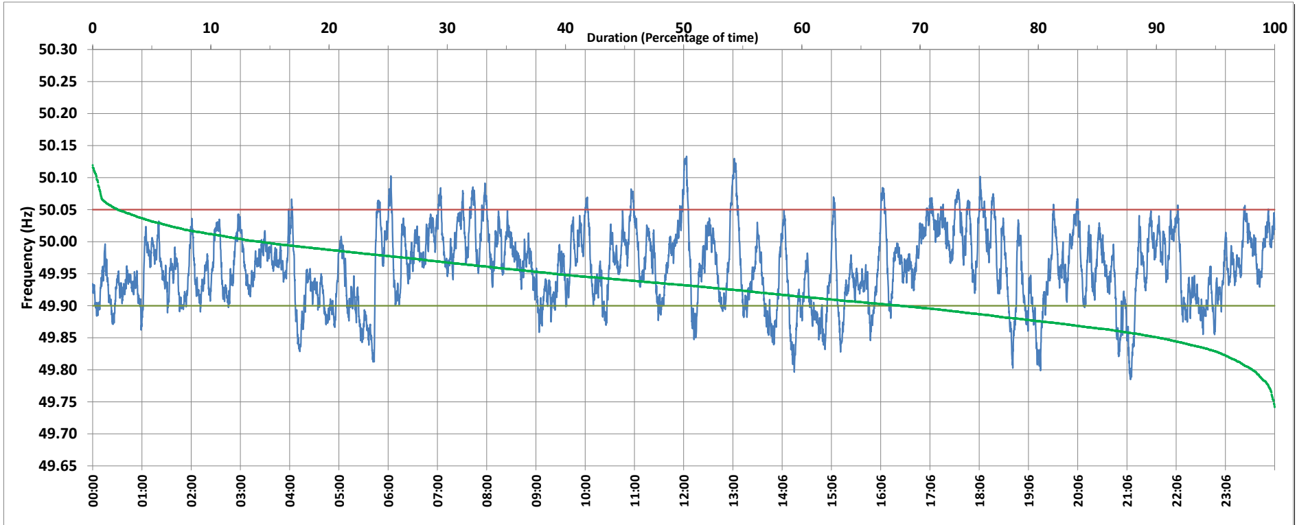
Frequency profile for 02-Jan-2019 (Wednesday)
