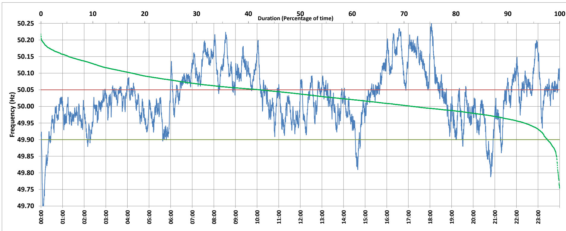
Frequency profile for 02-Jun-2019 (Sunday)
