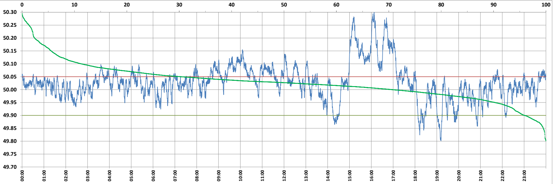
Frequency profile for 03-Jul-2022 (Sunday)
