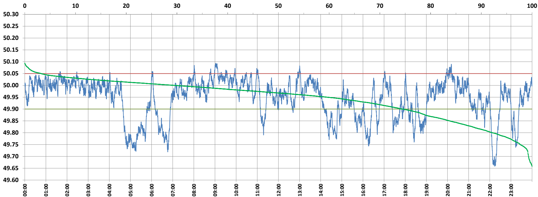
Frequency profile for 05-Oct-2021 (Tuesday)
