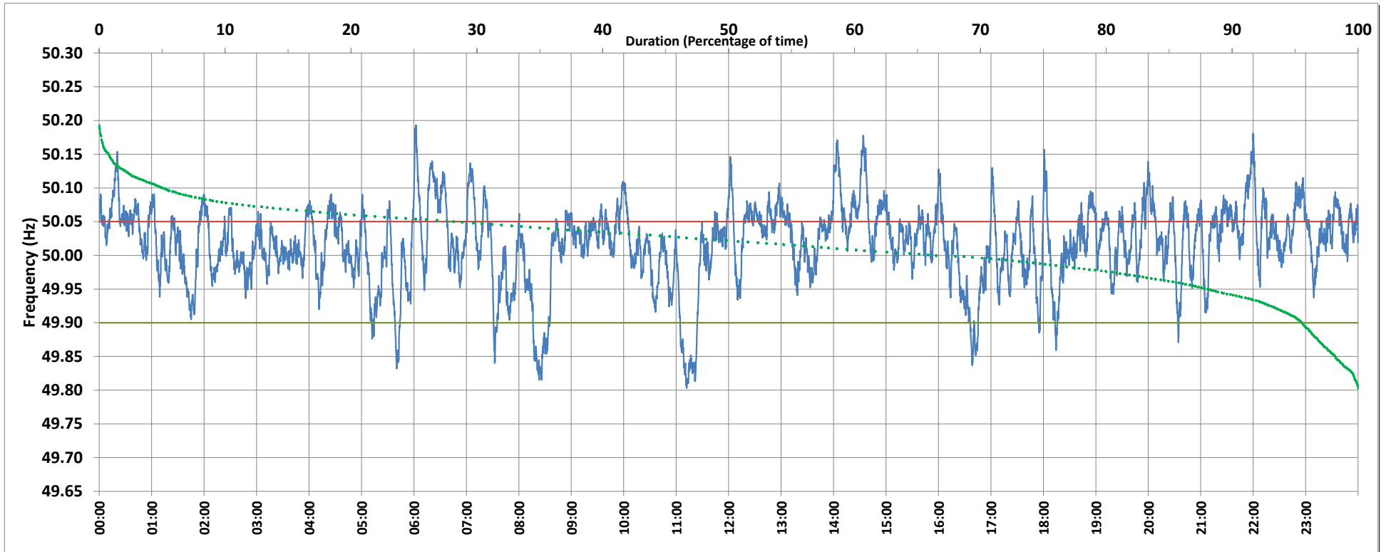
Frequency profile for 06-Jan-2019 (Sunday)
