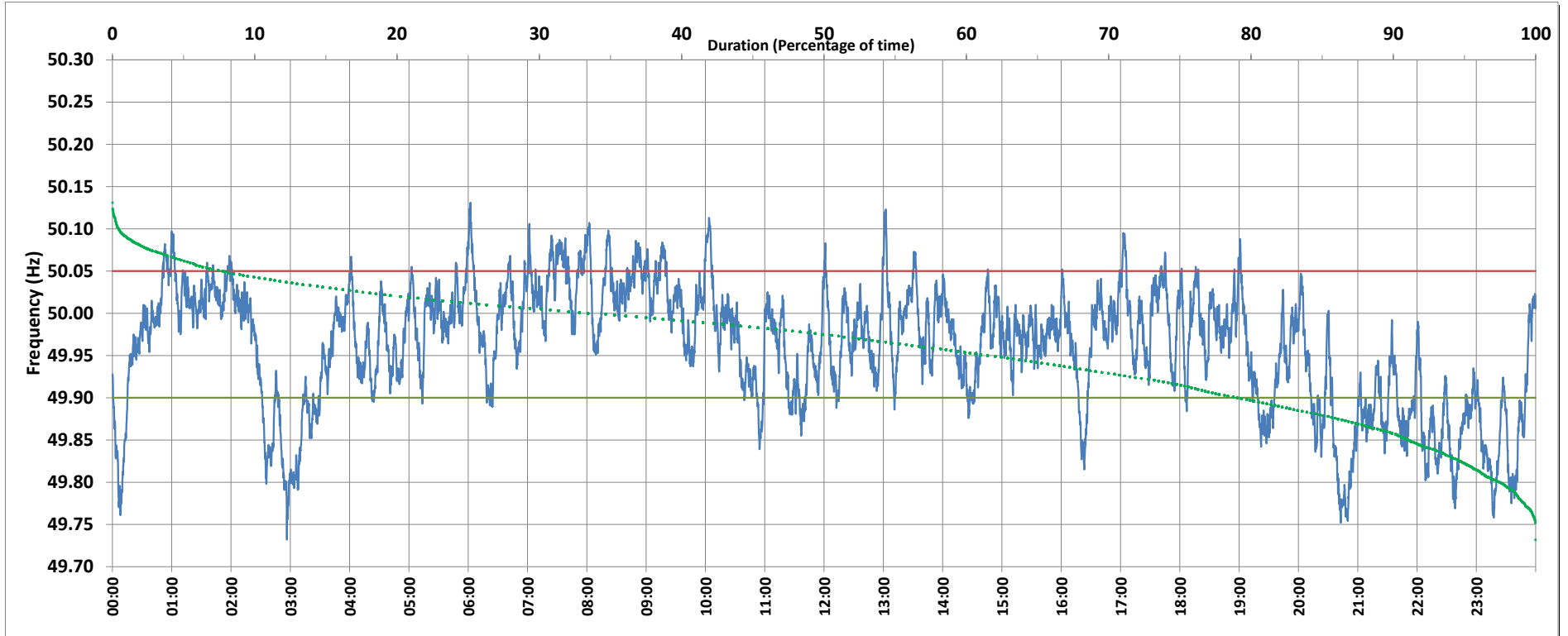
Frequency profile for 08-May-2019 (Wednesday)
