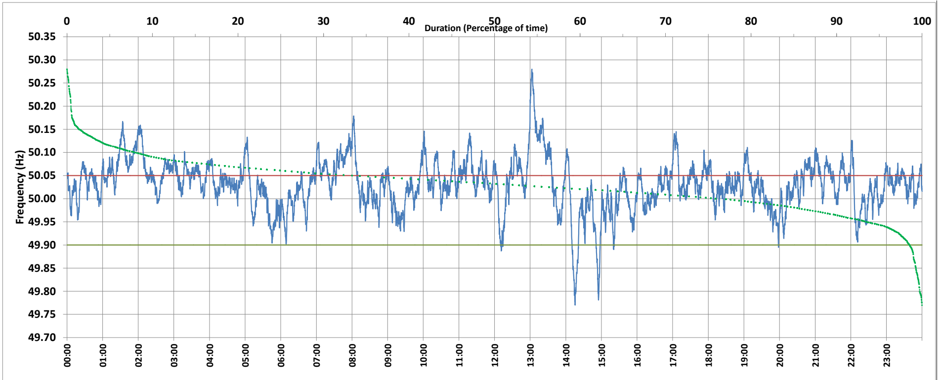
Frequency profile for 09-Jul-2019 (Tuesday)
