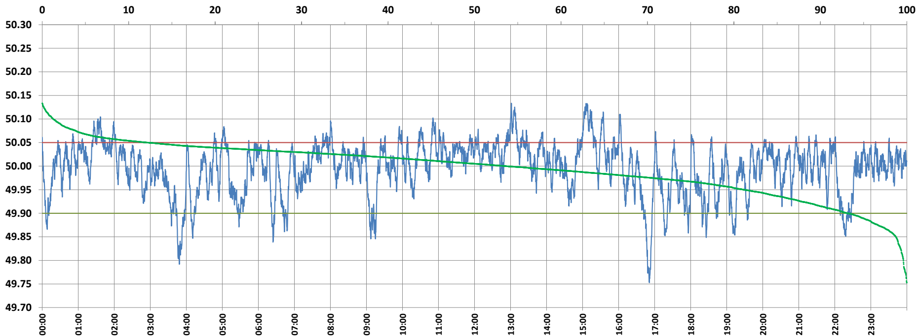
Frequency profile for 09-Sep-2021 (Thursday)
