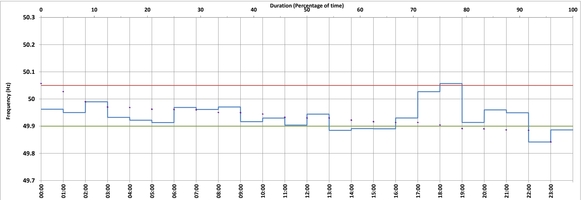
Hourly Average Frequency Profile for 11-May-2018
