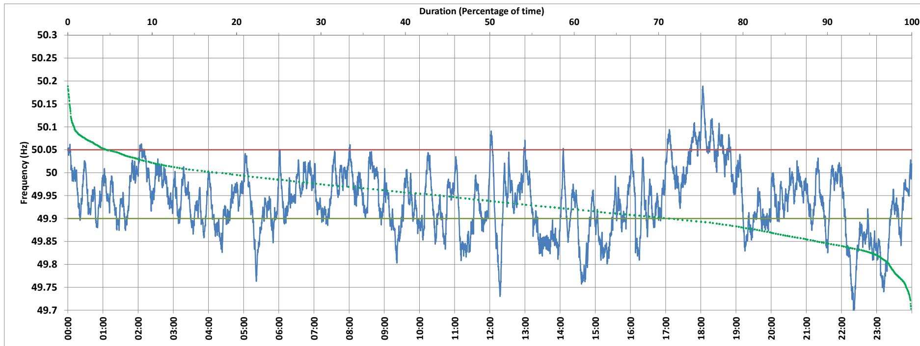
National Grid Frequency Profile for 11-May-2018
