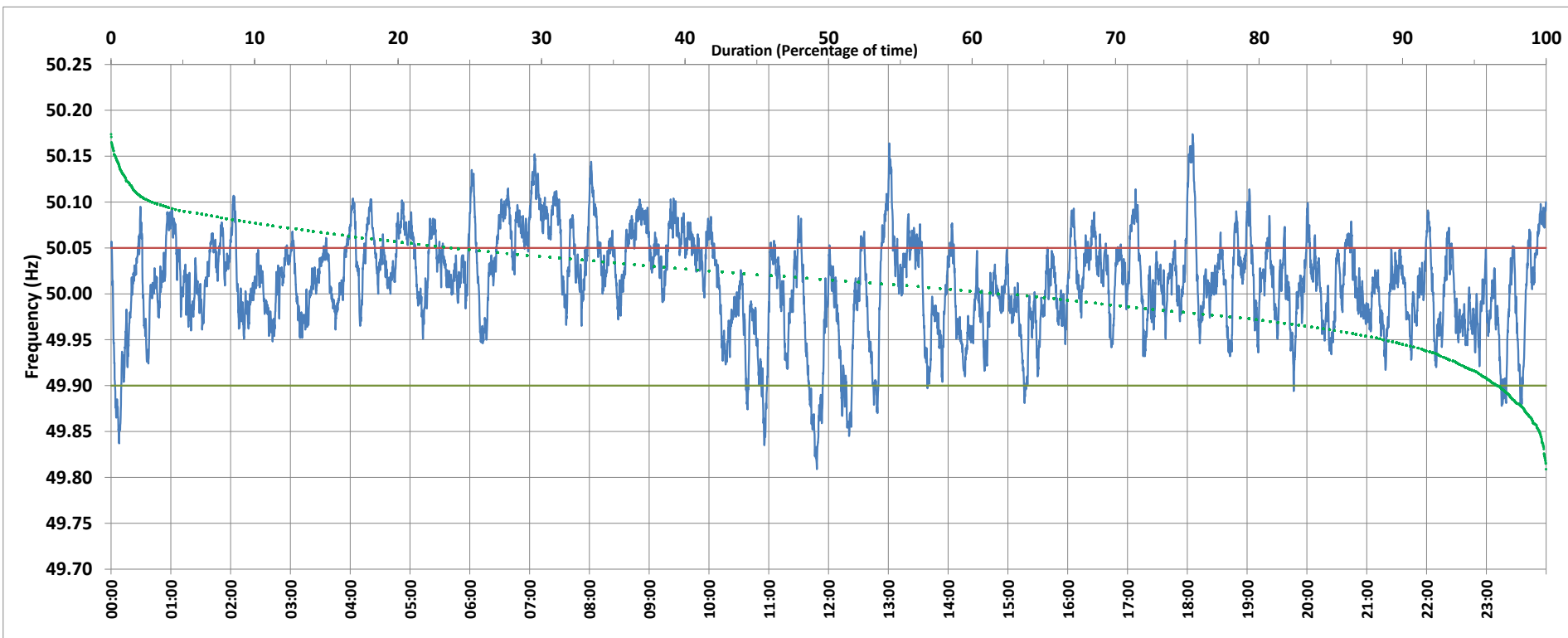
Frequency profile for 13-Jul-2019 (Saturday)
