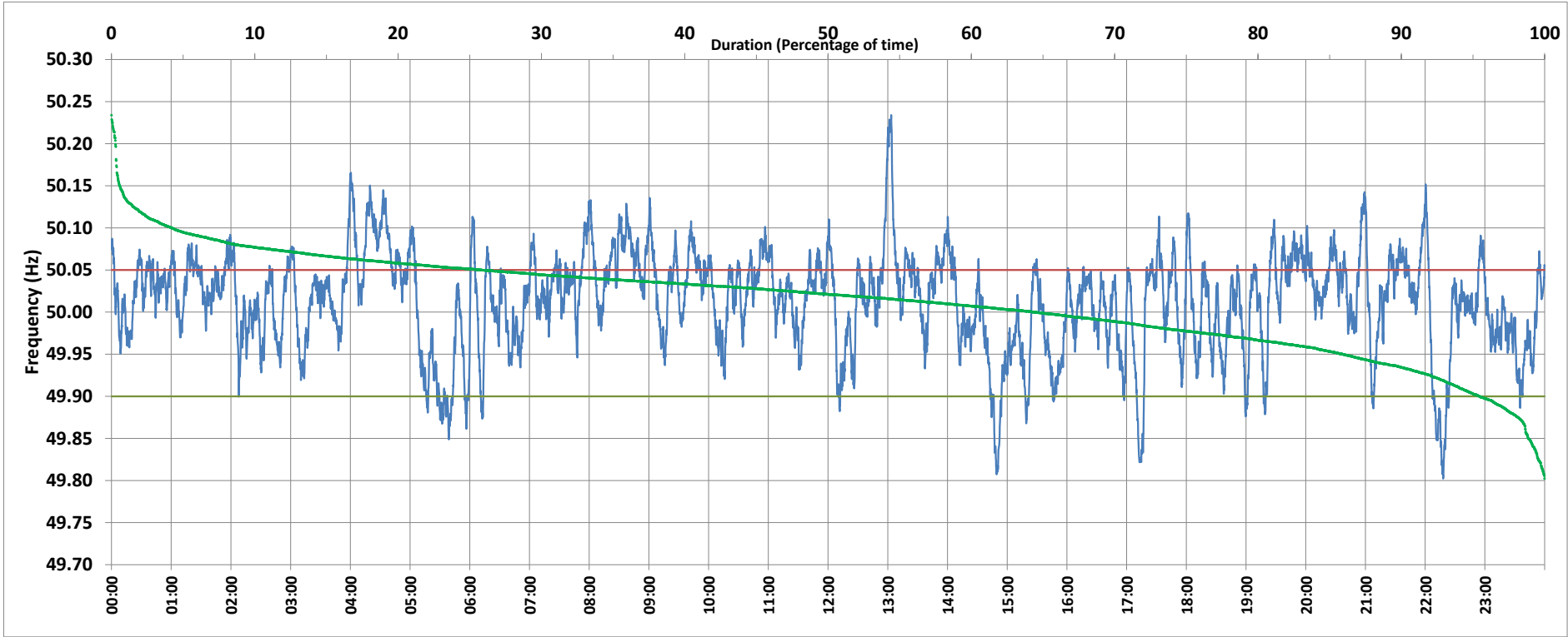
Frequency profile for 16-Mar-2019 (Saturday)
