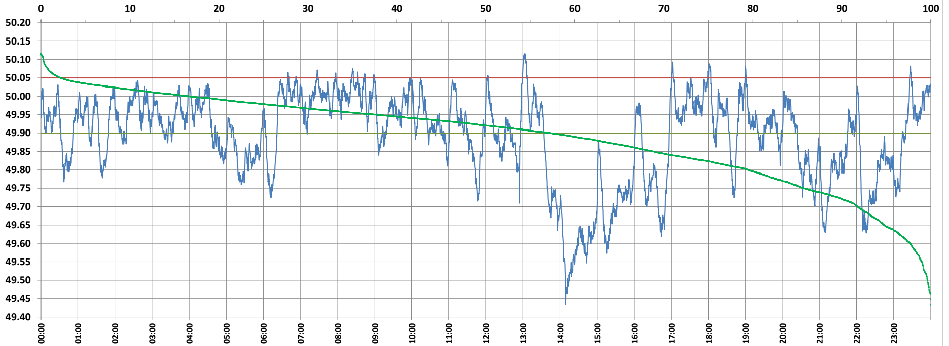
Frequency profile for 19-Apr-2022 (Tuesday)
