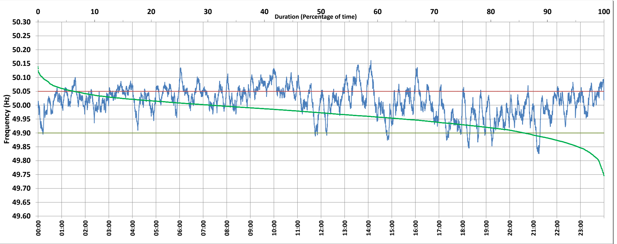
Frequency profile for 22-Jul-2018 (Sunday)
