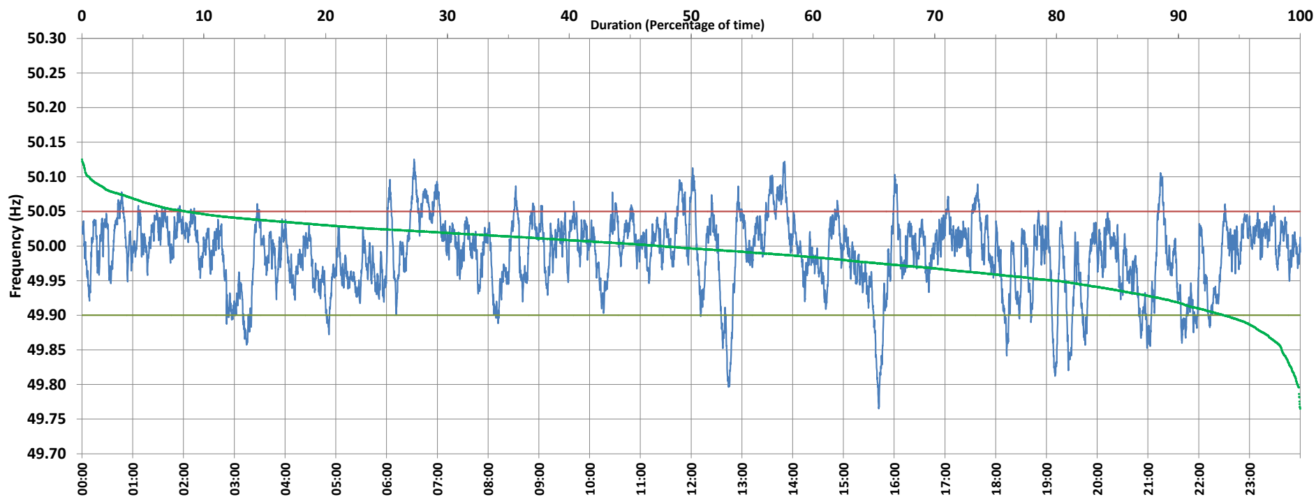
Frequency profile for 25-Jul-2020 (Saturday)
