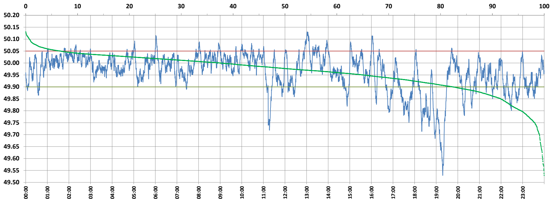
Frequency profile for 26-Aug-2021 (Thursday)
