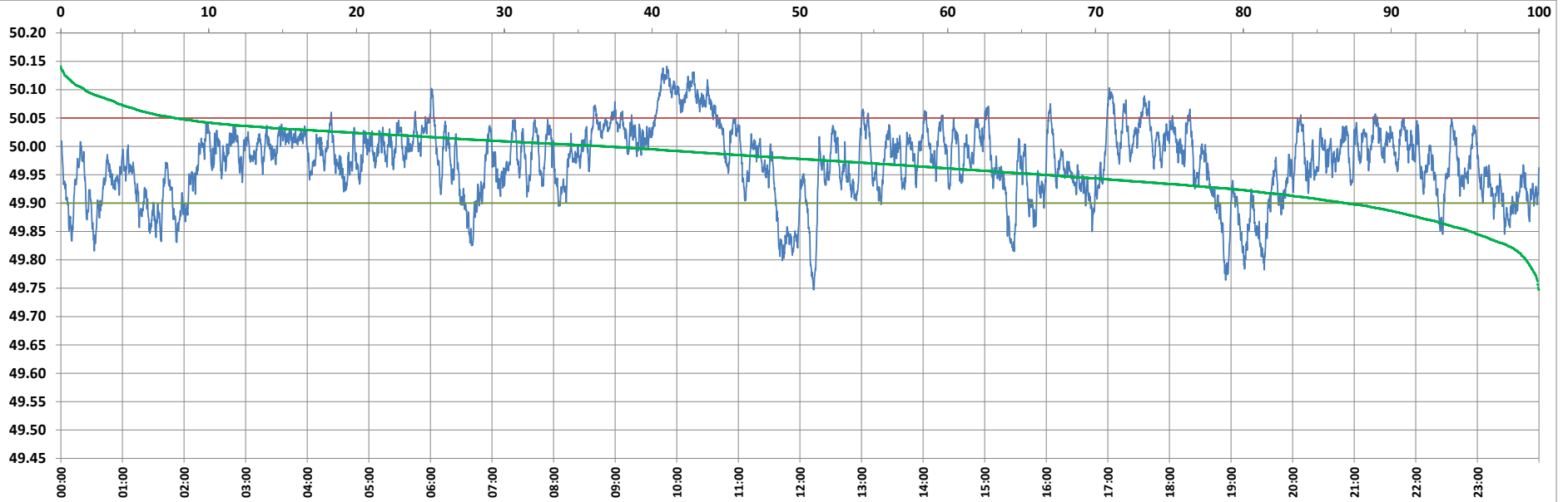
Frequency profile for 27-Aug-2022 (Saturday)
