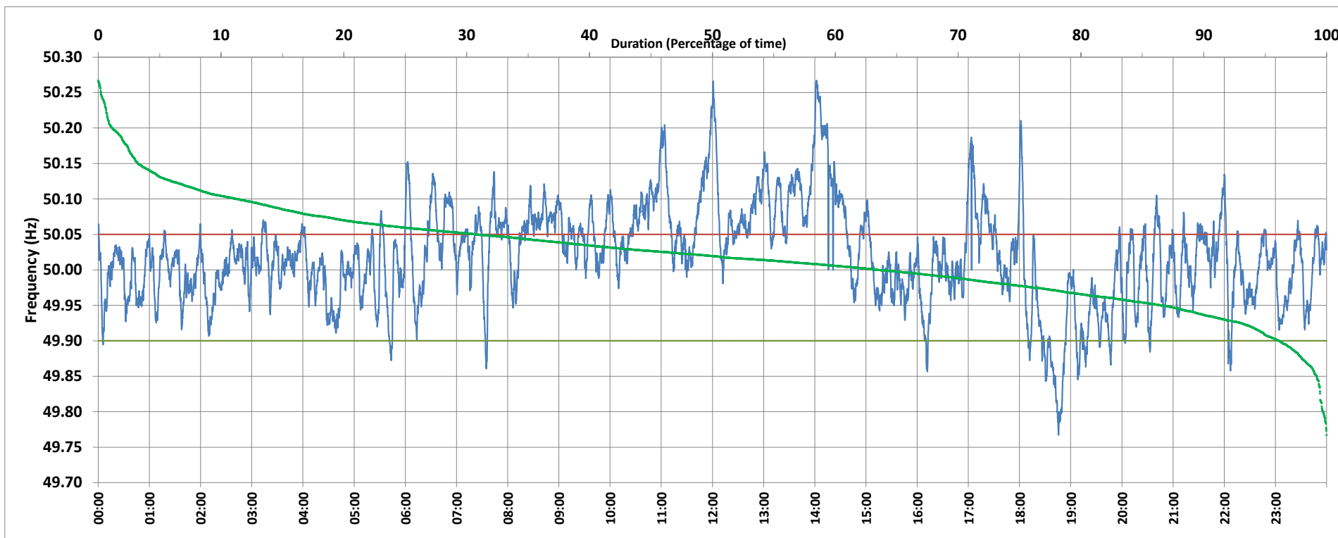
Frequency profile for 28-Mar-2020 (Saturday)
